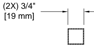
Towel Bar Cross Section Thickness .025"
